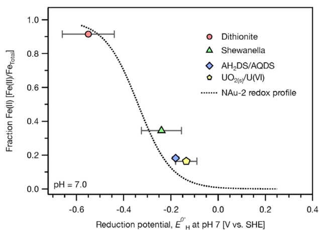
Figure 5. Measured fractions of Fe(II) vs reported standard state reduction potential values at pH 7.0 ( E^\circ_{\text{H}} ) for the four reductants investigated in this study. The reduction potential values were calculated from literature sources in Table 3. Error bars represent the reported range of E^\circ_{\text{H}} values. The dashed line is the fitted E^\circ_{\text{H}} profile for clay-Fe(II/III) in nontronite NAu-2 as determined by mediated electrochemical reduction. 20
